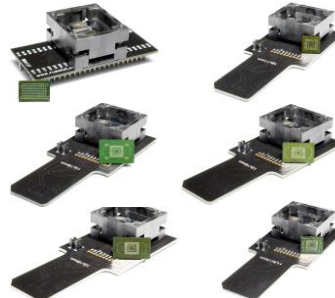
VNR Smartphone Kit BGA137, and various BGA169e adapters with sockets
