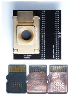
Monolithic NAND Adapter with Socket for microSD 6x4 pads
