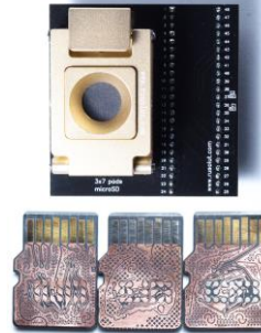
Monolithic NAND Adapter with Socket for microSD 3x7 pads
