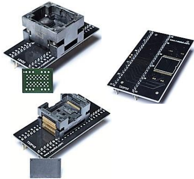
TLGA52 and TSOP56 ZIF adapters, and the TSOP48 adapter
