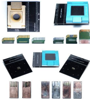
Monolithic NAND Adapters for monoUFD 6*6 & 3*7 pads, monoSD 3*13 pads, and Sandisk monoSD
